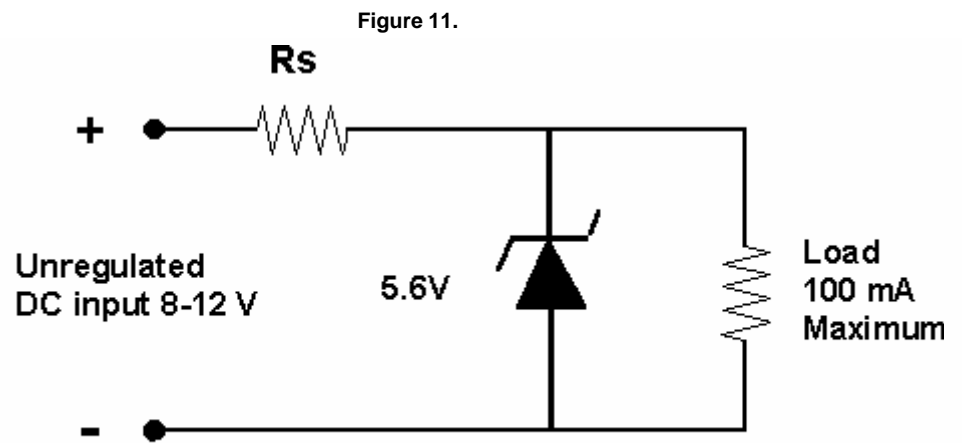
Zener diode used as shunt voltage regulator
